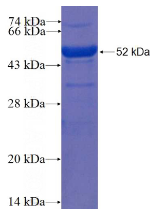
Recombinant Human PLEKHB2 SDS-PAGE
