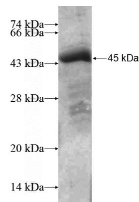
Recombinant Human NUDT11 SDS-PAGE
