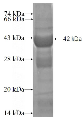
Recombinant Human RGS13 SDS-PAGE
