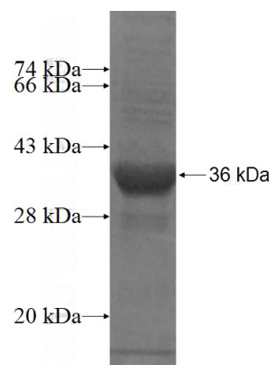
Recombinant Human NA14 SDS-PAGE
