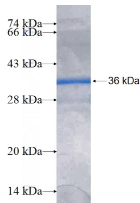
Recombinant Human VAMP8 SDS-PAGE
