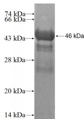
Recombinant Human HOOK2 SDS-PAGE
