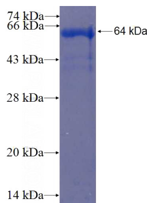
Recombinant Human PRDM8 SDS-PAGE
