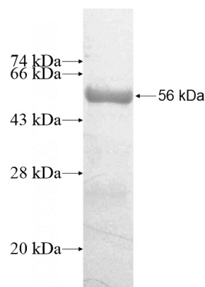
Recombinant Human OLAH SDS-PAGE
