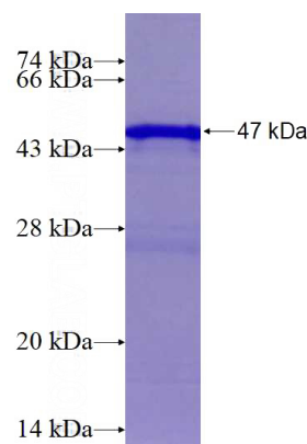
Recombinant Human RAB33A SDS-PAGE
