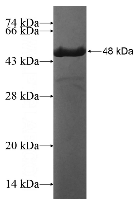
Recombinant Human LOH12CR1 SDS-PAGE
