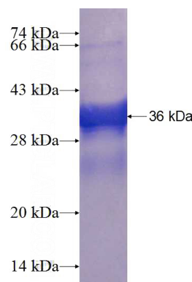
Recombinant Human L3MBTL4 SDS-PAGE
