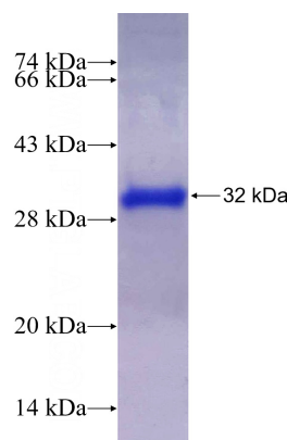
Recombinant Human TRIAP1 SDS-PAGE
