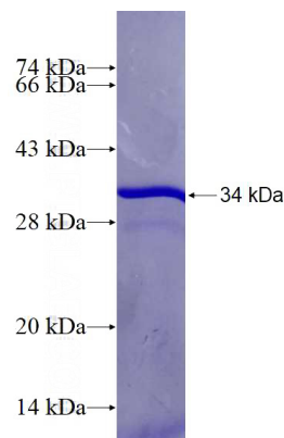
Recombinant Human ADIPOR1 SDS-PAGE
