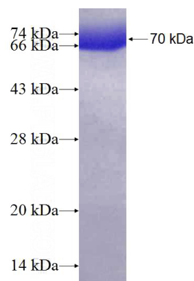
Recombinant Human dynactin-2 SDS-PAGE
