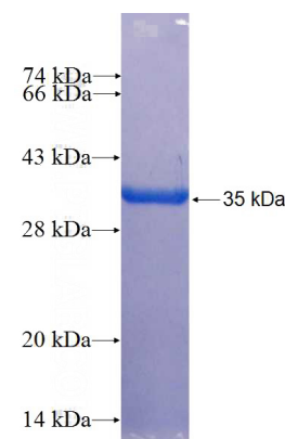
Recombinant Human NDNL2 SDS-PAGE
