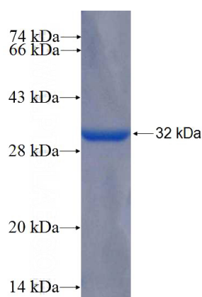
Recombinant Human FGF9 SDS-PAGE
