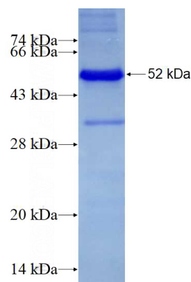
Recombinant Human LMCD1 SDS-PAGE
