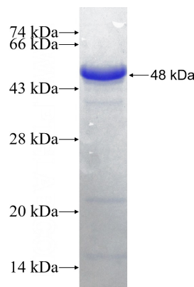
Recombinant Human NBR1 SDS-PAGE
