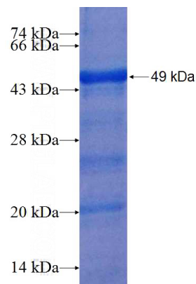
Recombinant Human REPS1 SDS-PAGE
