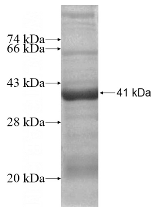
Recombinant Human TECPR2 SDS-PAGE
