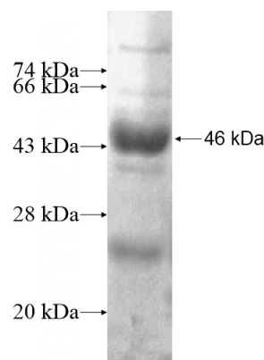
Recombinant Human PFTK2 SDS-PAGE
