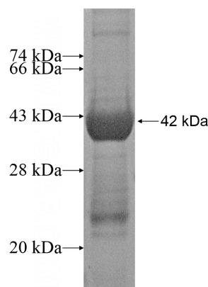
Recombinant Human SERPINB11 SDS-PAGE
