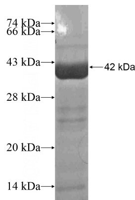
Recombinant Human MAOB SDS-PAGE
