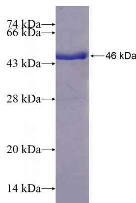
Recombinant Human TXNDC5 SDS-PAGE
