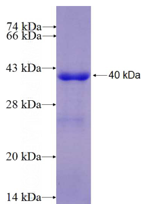
Recombinant Human PPP3CB SDS-PAGE
