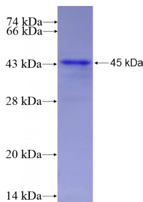
Recombinant Human INA SDS-PAGE
