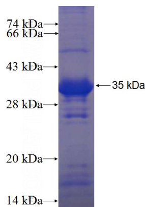
Recombinant Human CCDC137 SDS-PAGE
