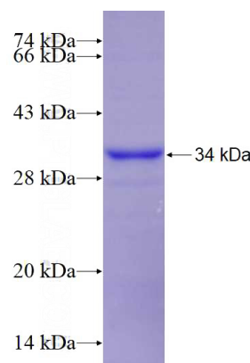
Recombinant Human VDAC3 SDS-PAGE
