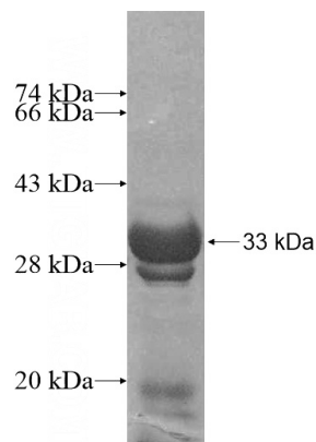
Recombinant Human UGT3A1 SDS-PAGE
