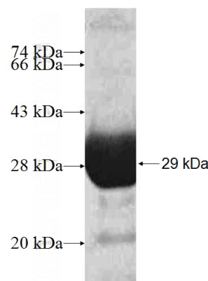
Recombinant Human AAK1 SDS-PAGE
