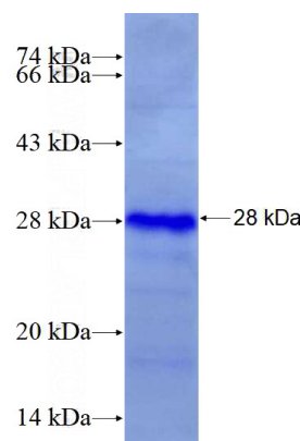
Recombinant Human EDN1 SDS-PAGE
