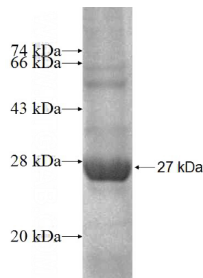
Recombinant Human NUP160 SDS-PAGE
