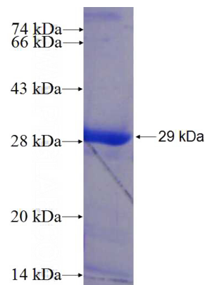
Recombinant Human DYDC2 SDS-PAGE
