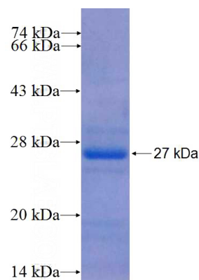
Recombinant Human C17orf57 SDS-PAGE
