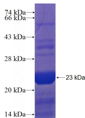
Recombinant Human AP1S2 SDS-PAGE
