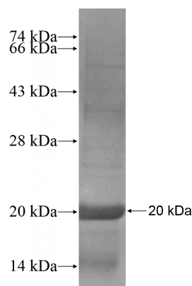
Recombinant Human COX5A SDS-PAGE
