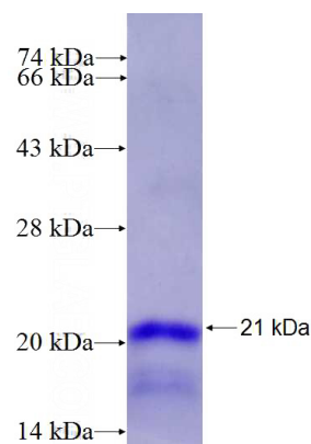
Recombinant Human ID2 SDS-PAGE
