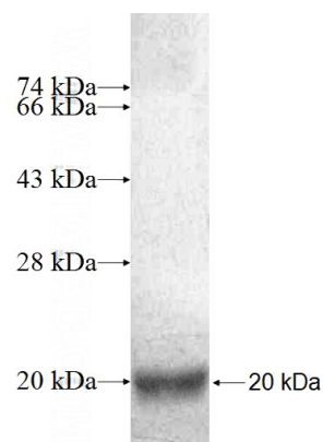
Recombinant Human H2AFV SDS-PAGE
