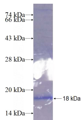
Recombinant Human SPAG11A SDS-PAGE
