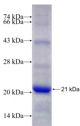
Recombinant Human TCEB2 SDS-PAGE
