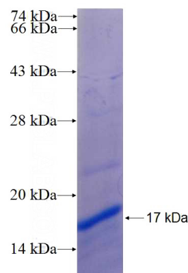
Recombinant Human SCAMP3 SDS-PAGE
