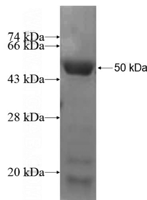
Recombinant Human FBX4 SDS-PAGE
