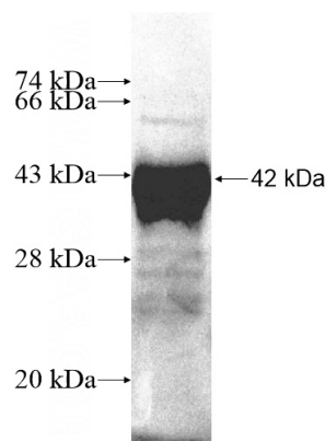
Recombinant Human ZFP28 SDS-PAGE
