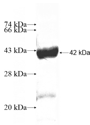
Recombinant Human CSGLCA-T SDS-PAGE
