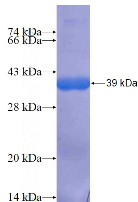
Recombinant Human USP3 SDS-PAGE
