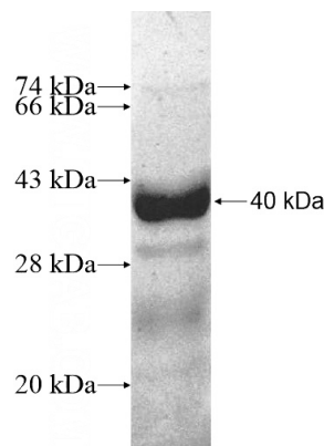
Recombinant Human STX19 SDS-PAGE
