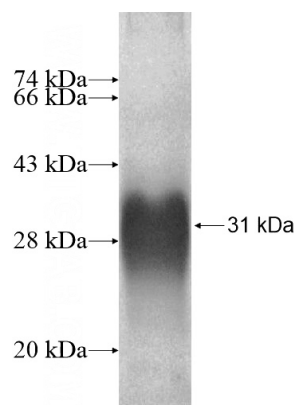
Recombinant Human KCNC4 SDS-PAGE
