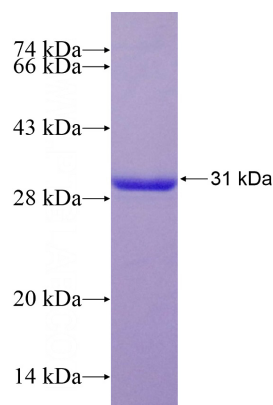
Recombinant Human ALKBH7 SDS-PAGE
