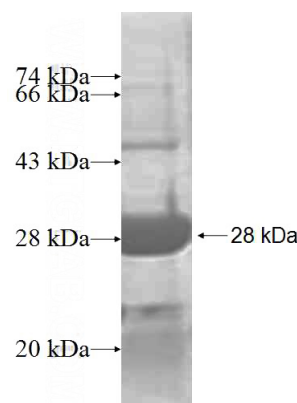
Recombinant Human ARL4D SDS-PAGE
