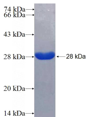
Recombinant Human CHMP1B SDS-PAGE
